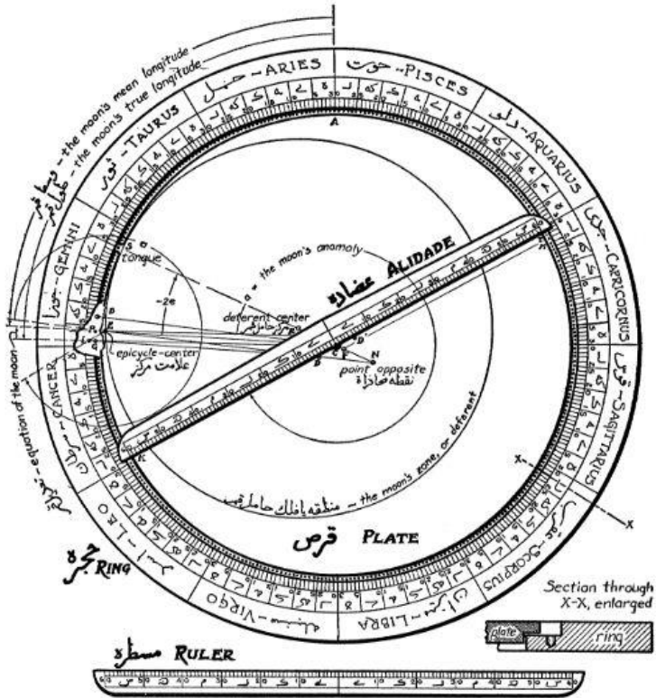
Gambar 3.1. bidang thabaq al-manatiq
