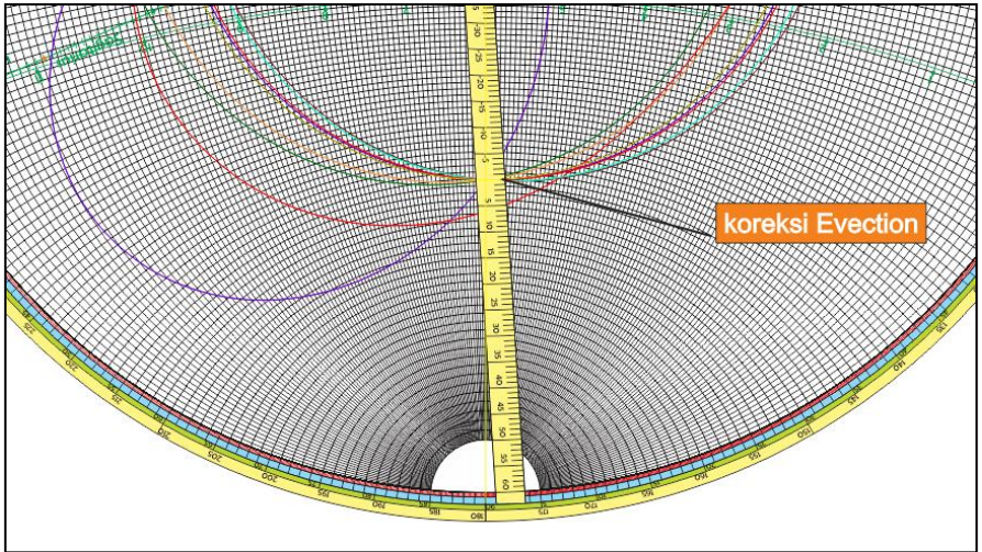
Gambar 4.12. Mencari Koreksi Evection
