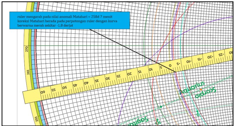
Gambar 4.7. Koreksi Equation of Center
