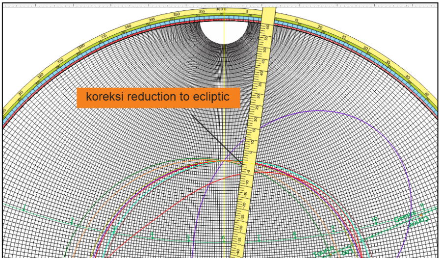
Gambar 4.15. Mencari Koreksi reduction to ecliptic
