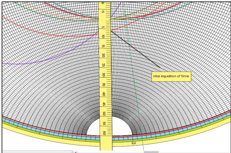
Gambar 4.9. Mencari Equation of time
