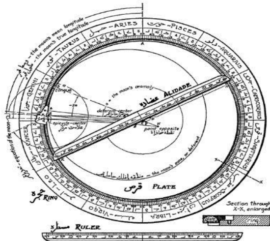
Gambar 1.1. Thabaq al-manatiq al-kashi.
