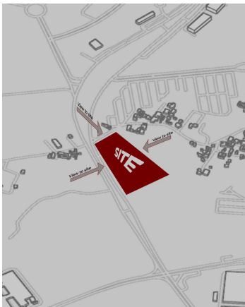
gambar 4.5. Analisa View
