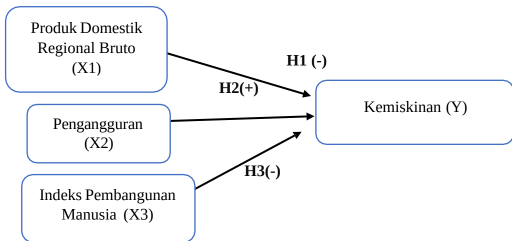
Gambar 2. 1 Model Penelitian
